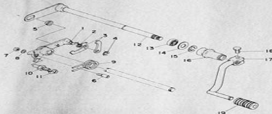
Fig. 1.10 Gearchange mechanism
