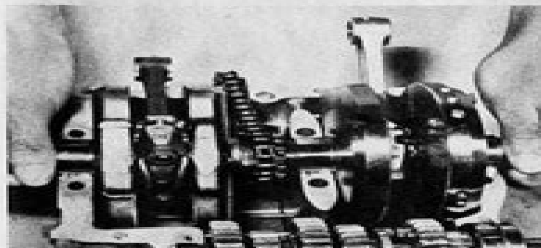
34.3 Lift crankshaft and cam chain into position in crankcase
