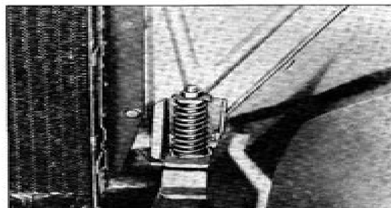
Fig. 5—1½ and 2 Ton Support Mounting
