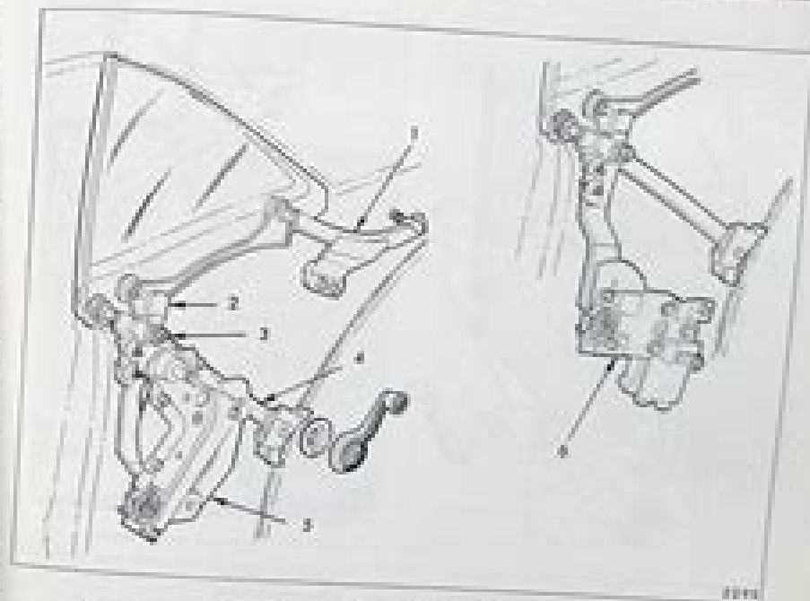
Fig. 1-12 Rear Quarter Window - "C" Style
