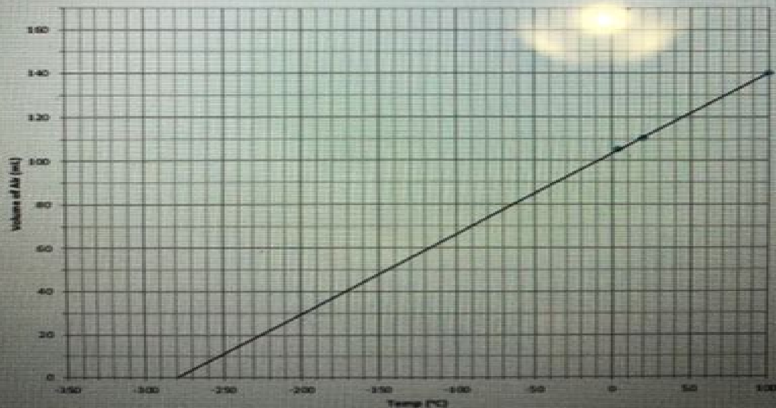
Volume of Air (mL) v Temperature (°C)
