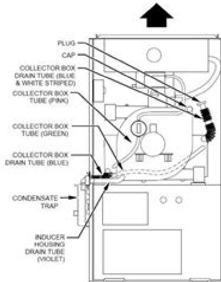
Fig. 6—Alternate Upflow Tube Configuration and Trap Location
