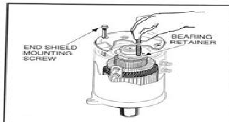
Figure 15-13 End Shield Installation
