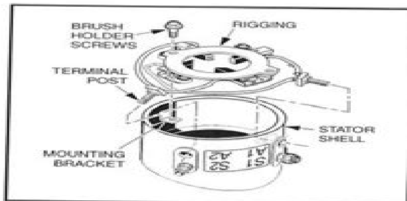
Figure 15-12 Brush Installation
