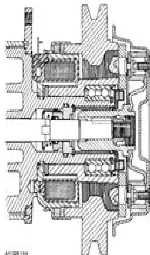
A/C CLUTCH
