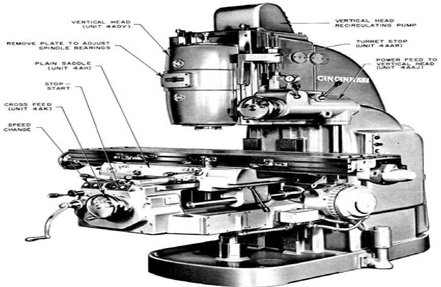
FIGURE 8 No. 3 Vertical Machine
