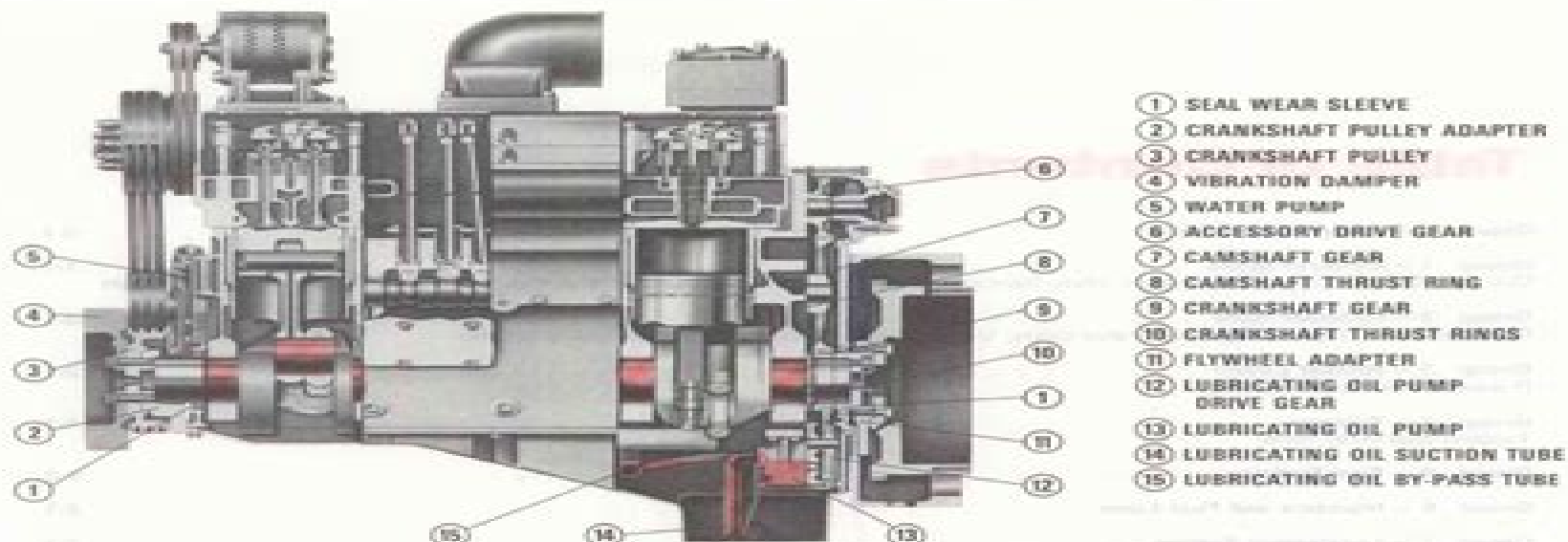
Fig. 7-6-1, (LWC-16). Lubricating oil and coolant flow.
