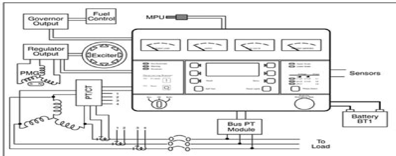
FIGURE 1-1. GENERATOR SET CONTROL FUNCTIONS
