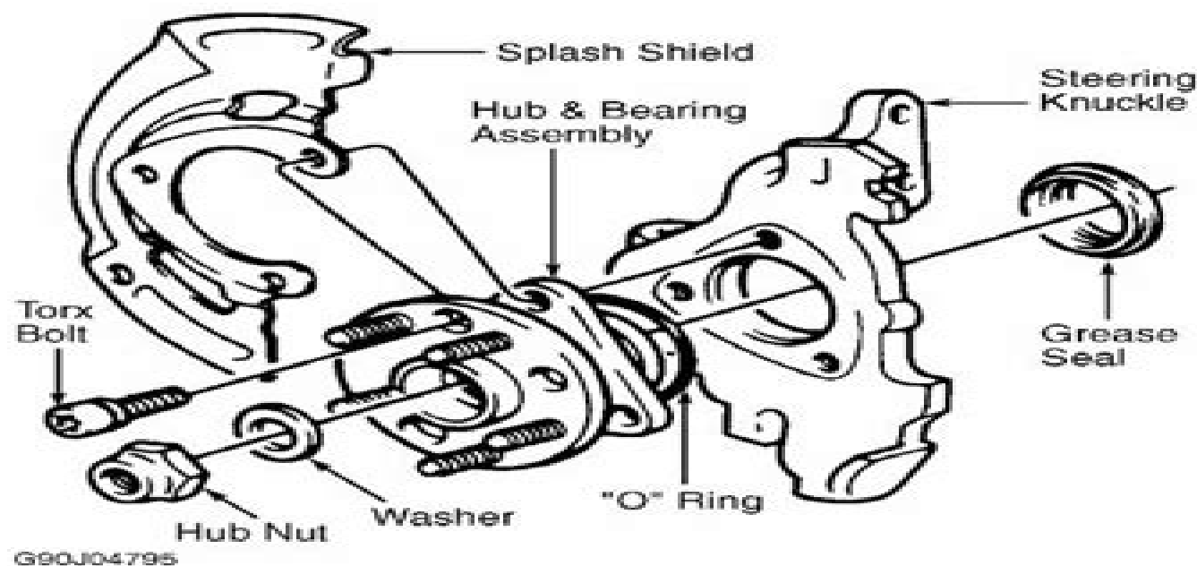
Fig. 3: Exploded View Of Hub & Bearing Assembly Courtesy of GENERAL MOTORS CORP.
