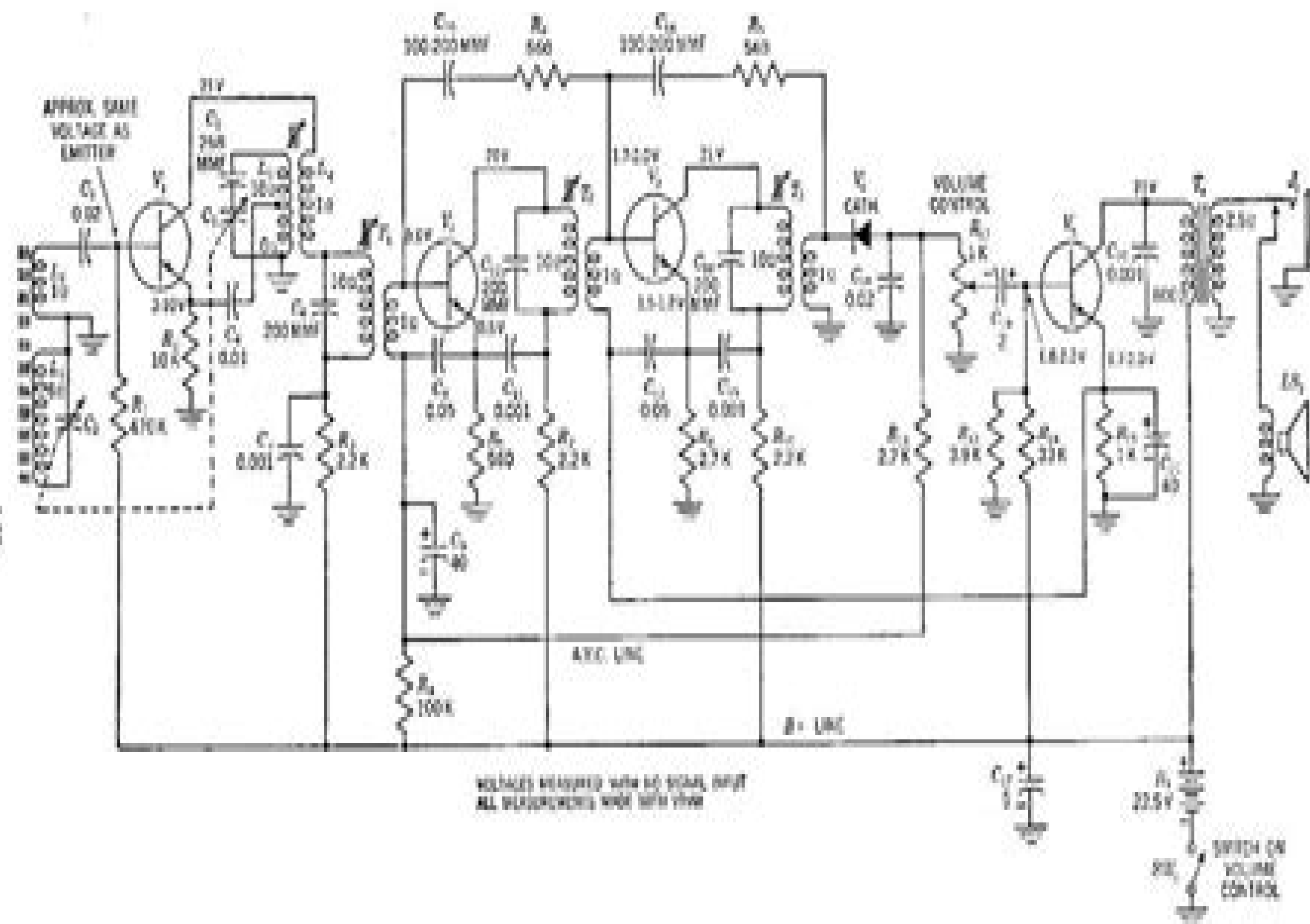
FIG. 3. The schematic diagram of the Regency model TR-1 receiver (Courtesy Howard W. Sams & Co., Inc.)
