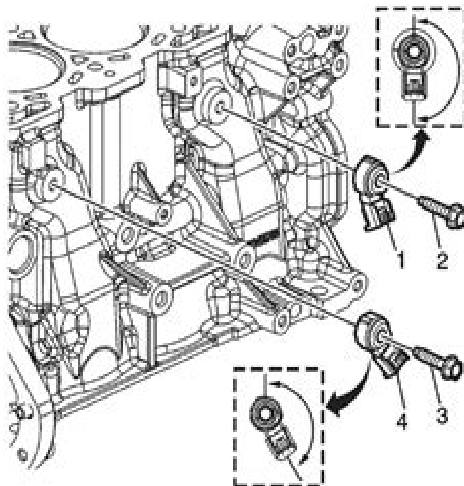
Fig. 213: Knock Sensor
