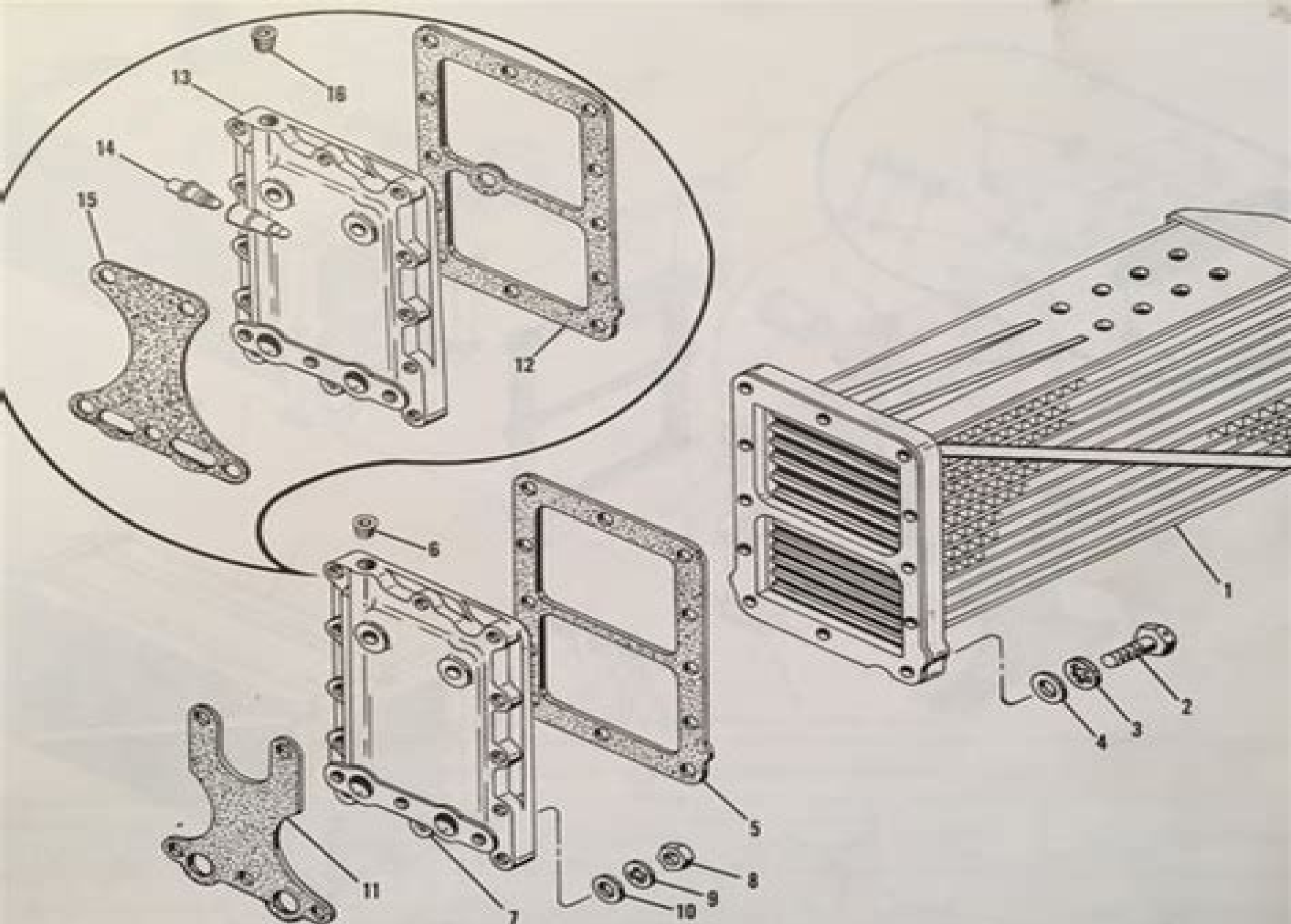
Figure 21. Oil Cooler Group (Models O-470-B, -M, and IO-470-D, -L, -M, and -U)
