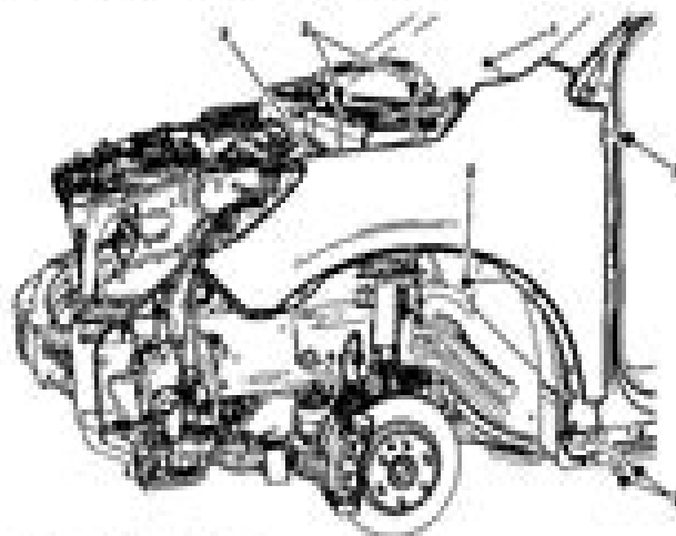
Fig. 7. Front Fender (Enclave) Courtesy of GENERAL MOTORS COMPANY
