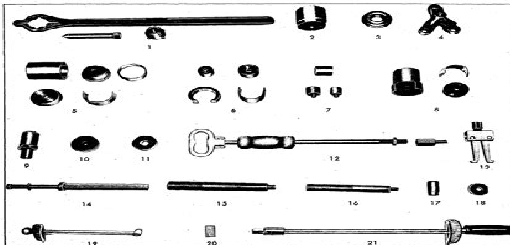
Fig. 113—Rear Suspension Special Tools (Chevrolet, Camaro, Chevelle and Chevy II)
