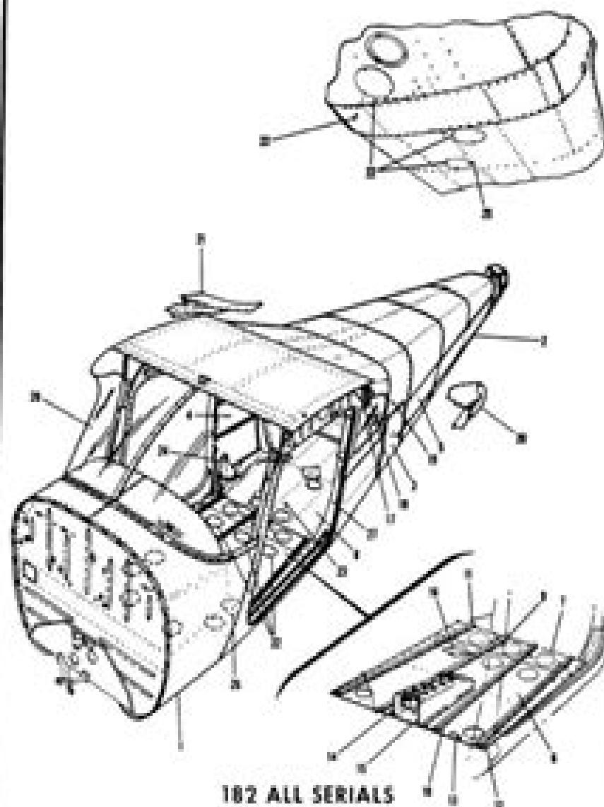
Figure 15. Fuselage Assembly
