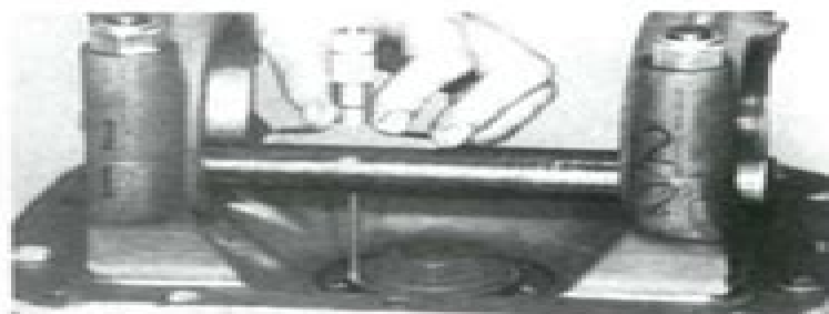
Fig. 29—View showing proper depth gage and pilot shaft placement used in determining pinion shaft protrusion.
