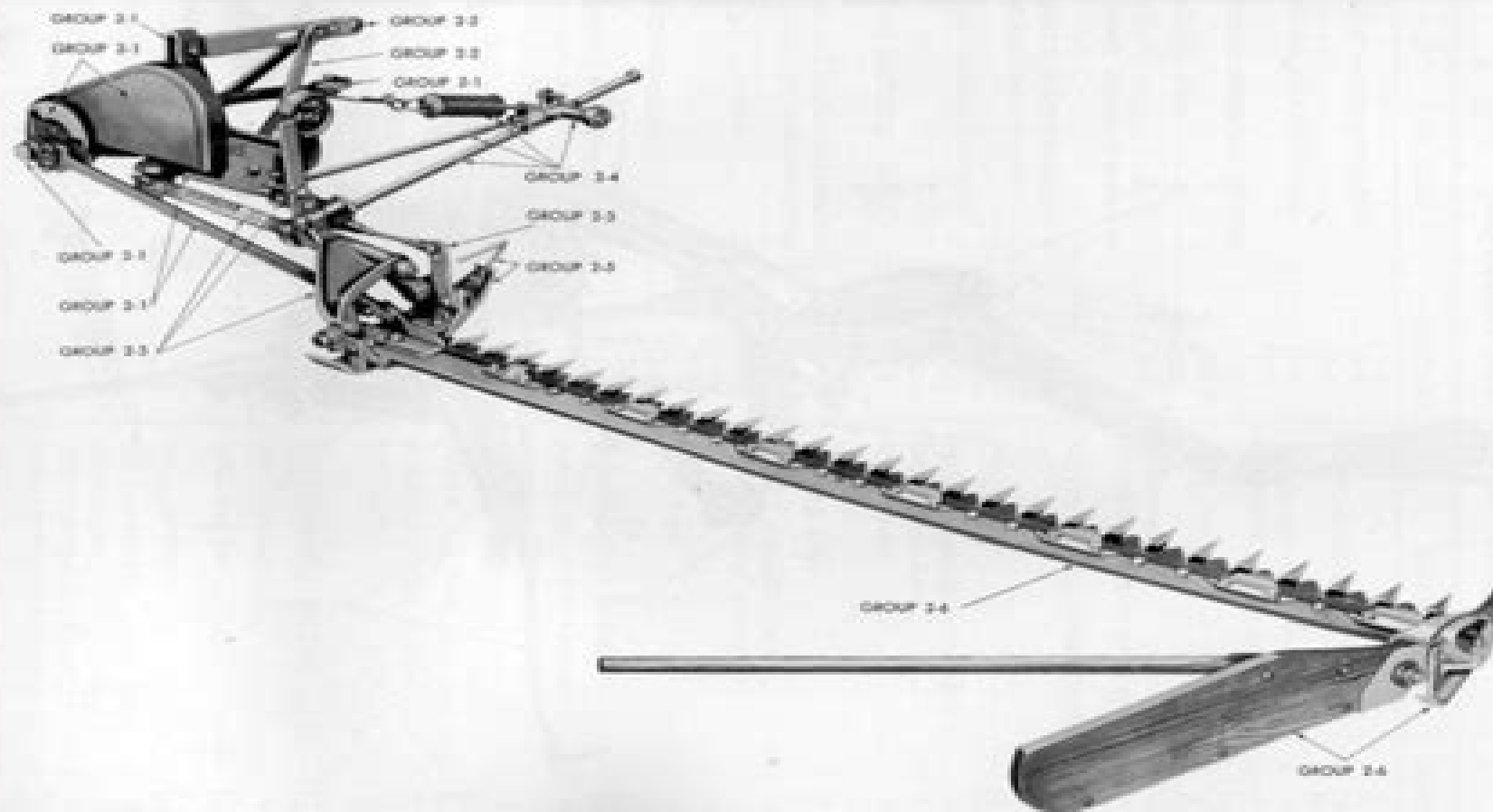
Figure 2 - Dearborn Rear Attached Mower (Models 14-16)
