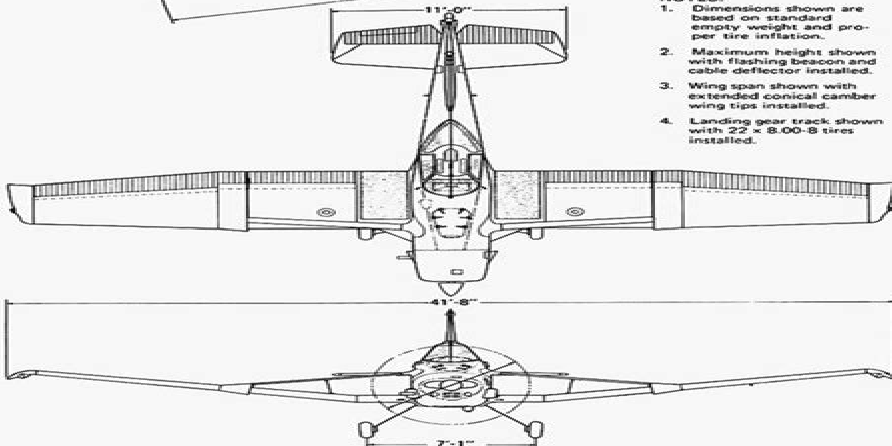
Principal Dimensions (Ag Truck Shown)
