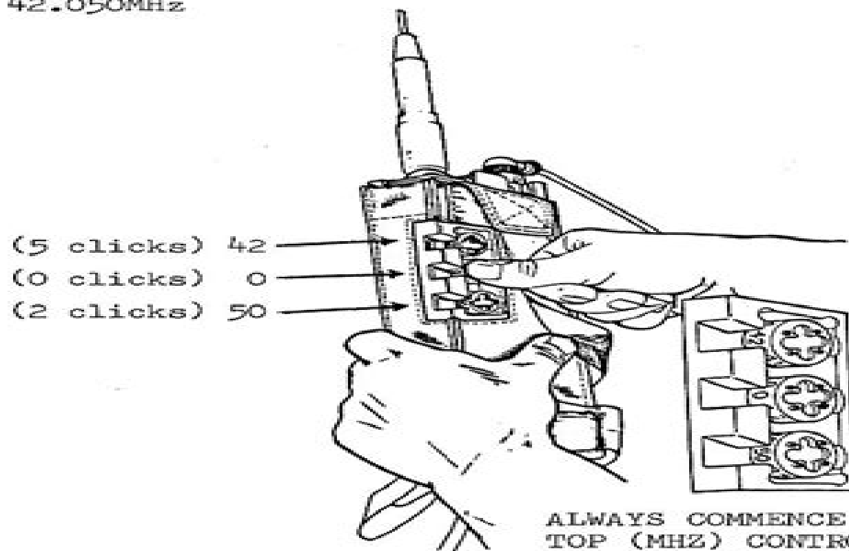
Fig 5 - Frequency Setting
