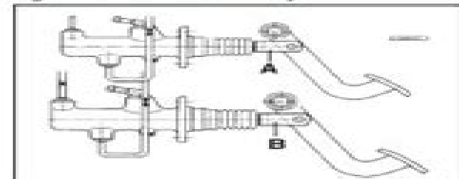
Fig. 14 - Adjusting the brake pedals.
