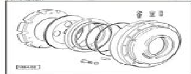
Fig. 13 - Rear brake assembly.
