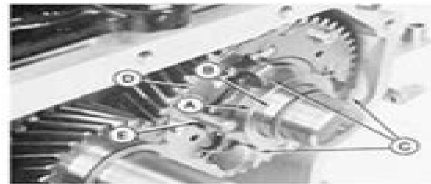
A—Governor Sleeve B—Camshaft C—Weights D—Weight Assembly Plate E—Locator Pin
