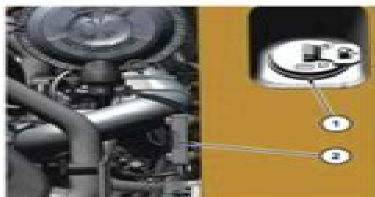
Illustration 2 g06325795 Type 2 Hydraulic Oil Level Gauge and Fill (1) Hydraulic Oil Fill (2) Hydraulic Oil Sight Gauge
