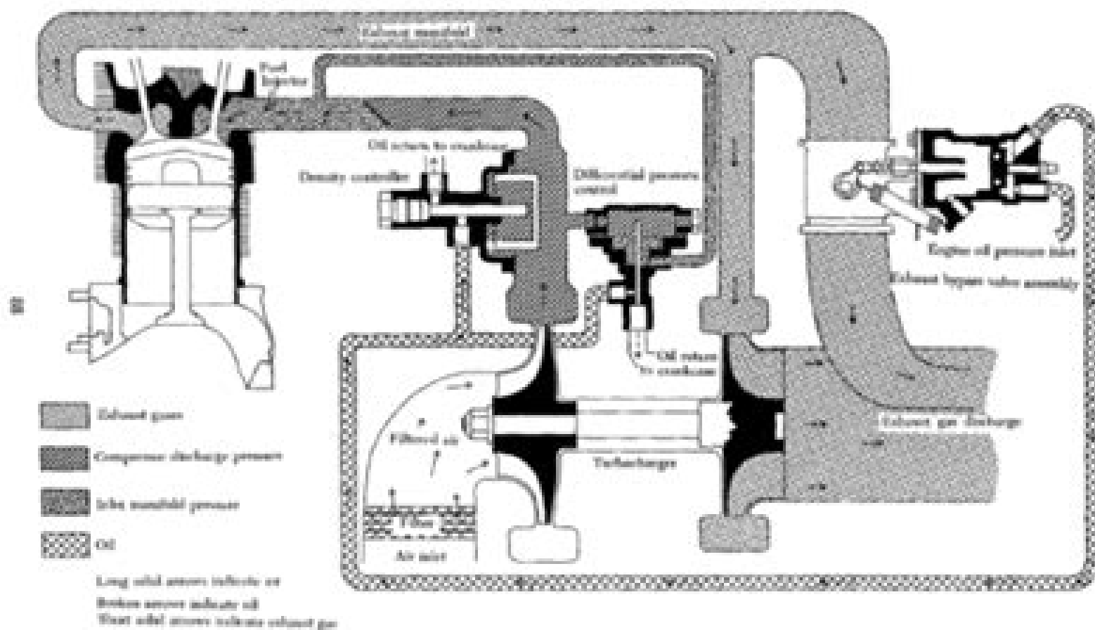
FIGURE 2-16. Turbocharger controller and waste-gas actuator system schematic.
