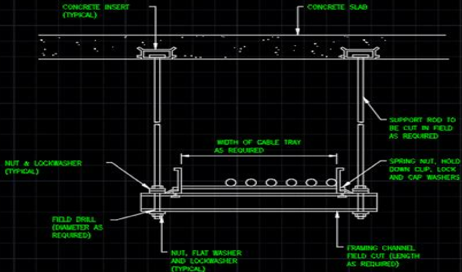
CABLE TRAY SUPPORT
