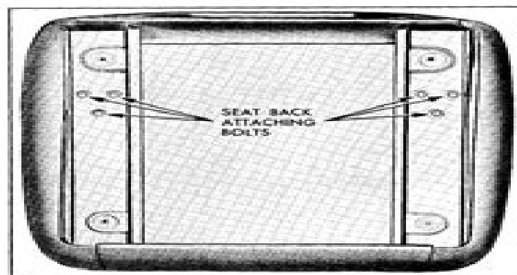
Fig. 15-77 Bucket Seat Back Attachment
