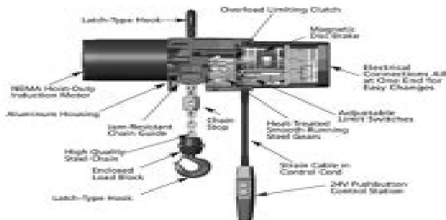
Figure 2 — Electric Hoist Construction
