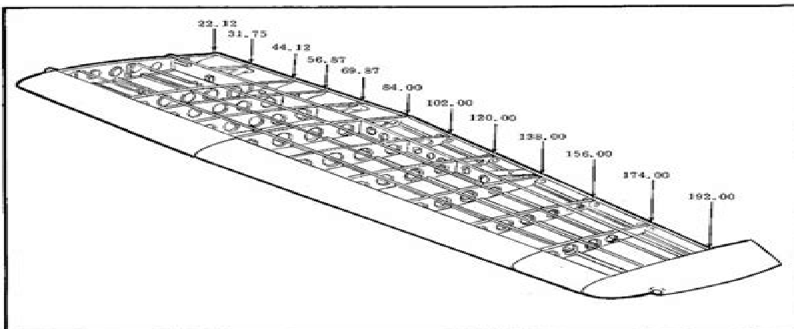
Figure 1-3. Wing Stations
