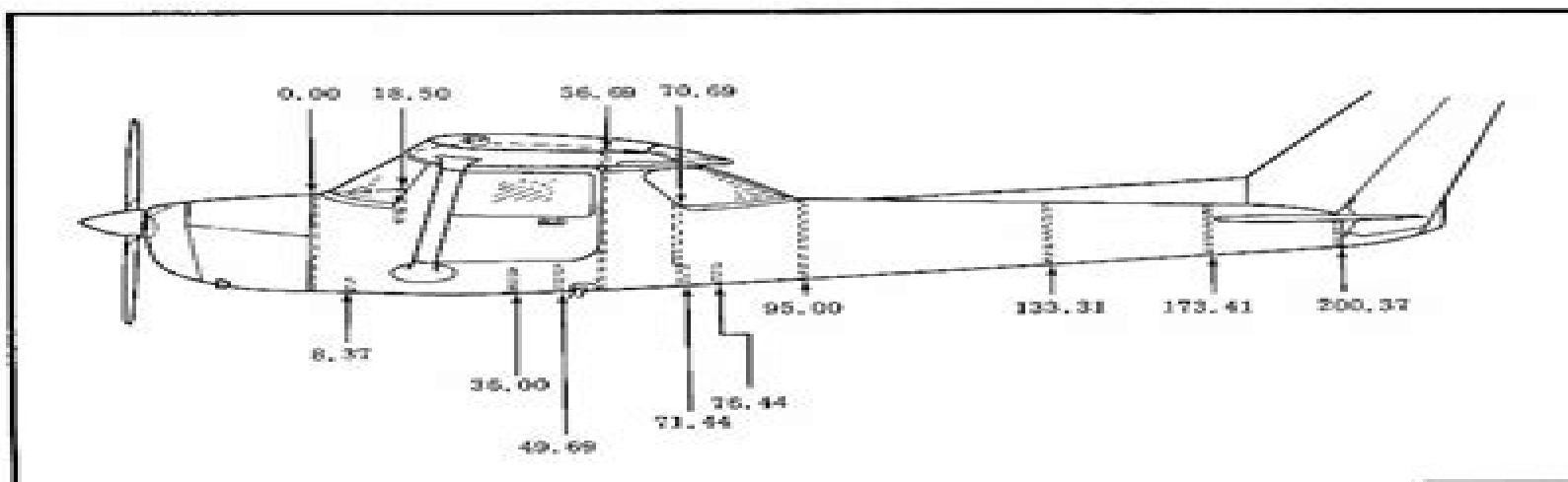
Figure 1-2. Fuselage Stations
