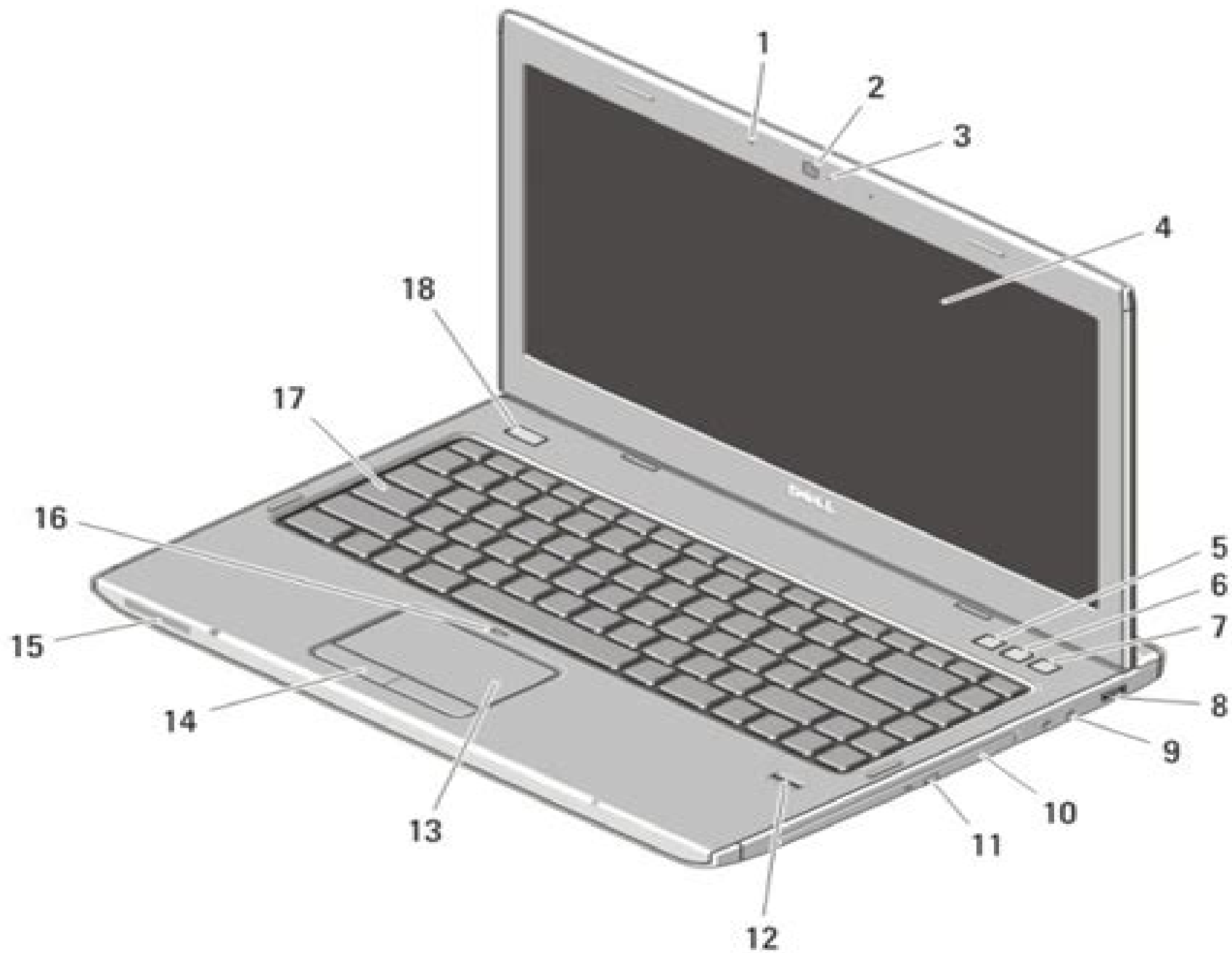
Figure 3. Vostro 3450 — Front view
