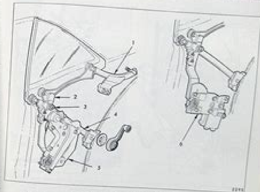
Fig. 1-12 Rear Quarter Window Regulator - 17" Style
