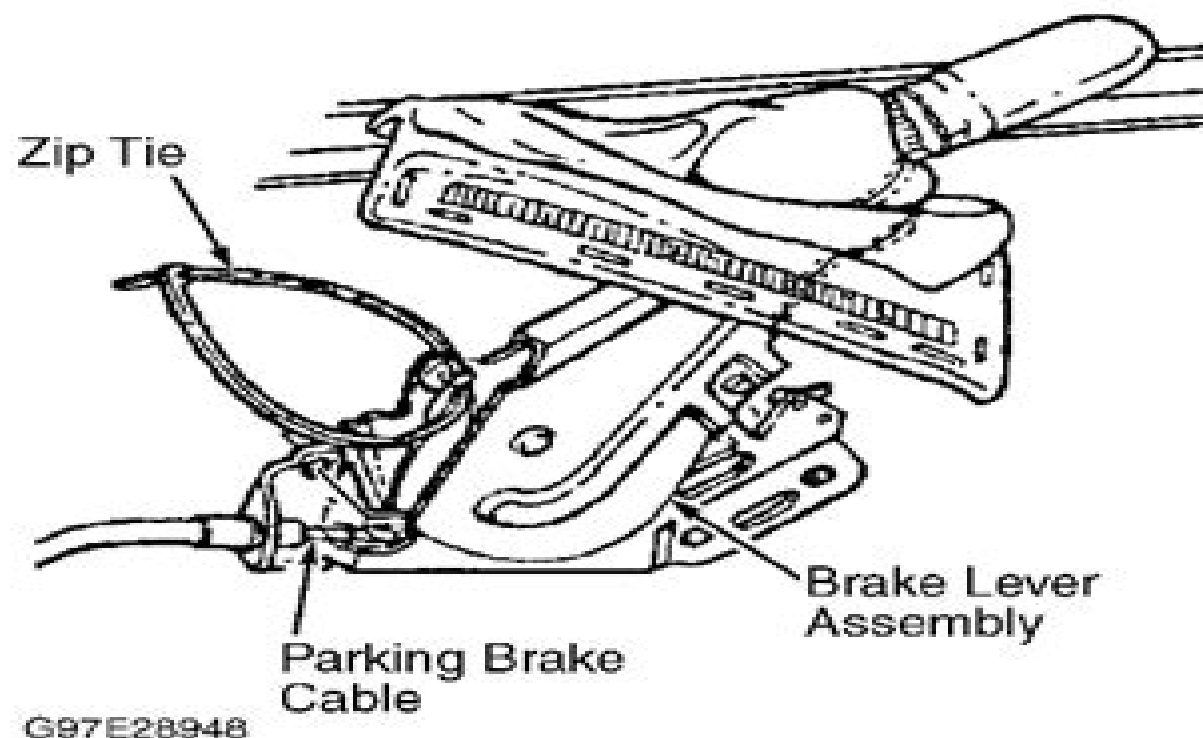
Fig. 1: Disabling & Enabling Parking Brake Cable Automatic Adjuster Courtesy of GENERAL MOTORS CORP.
