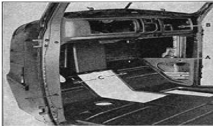
Fig. 1—Cowl and Dash Assembly
