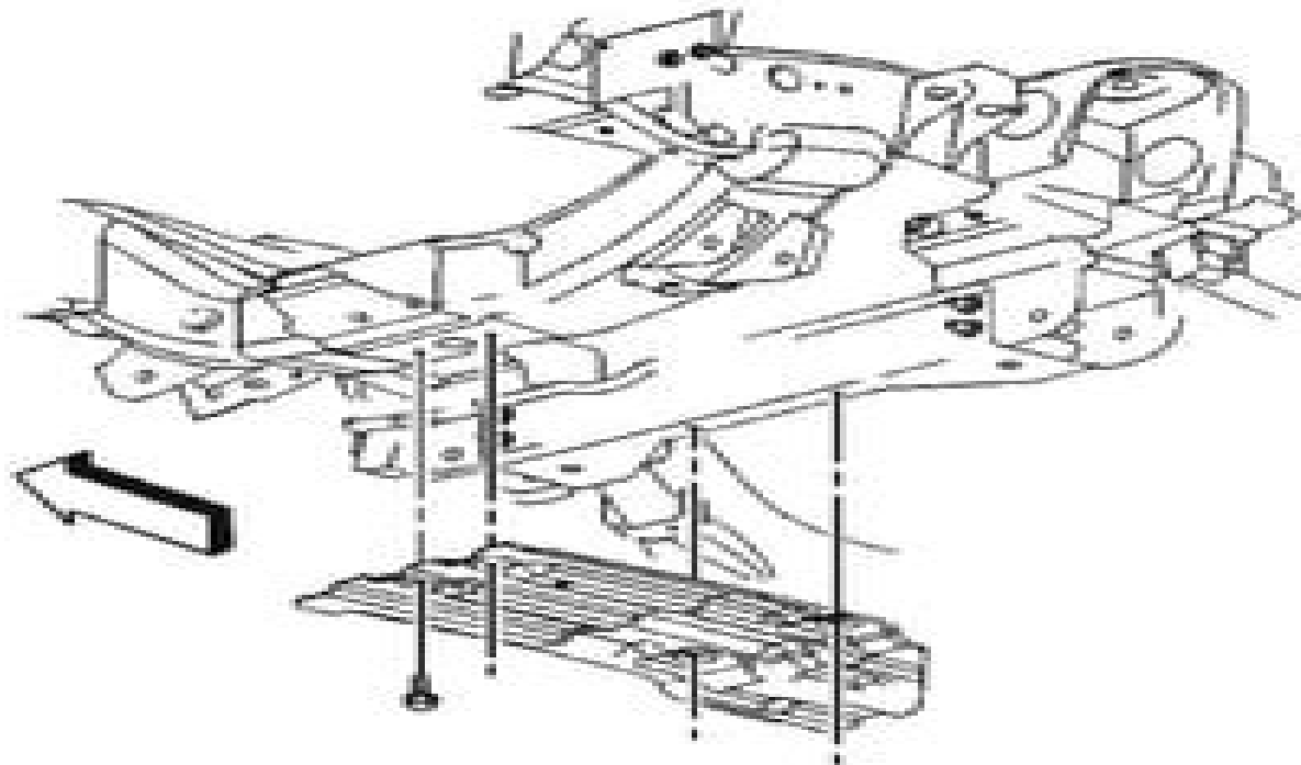
Fig. 7: Identifying Oil Pan Skid Plate Courtesy of GENERAL MOTORS CORP.
