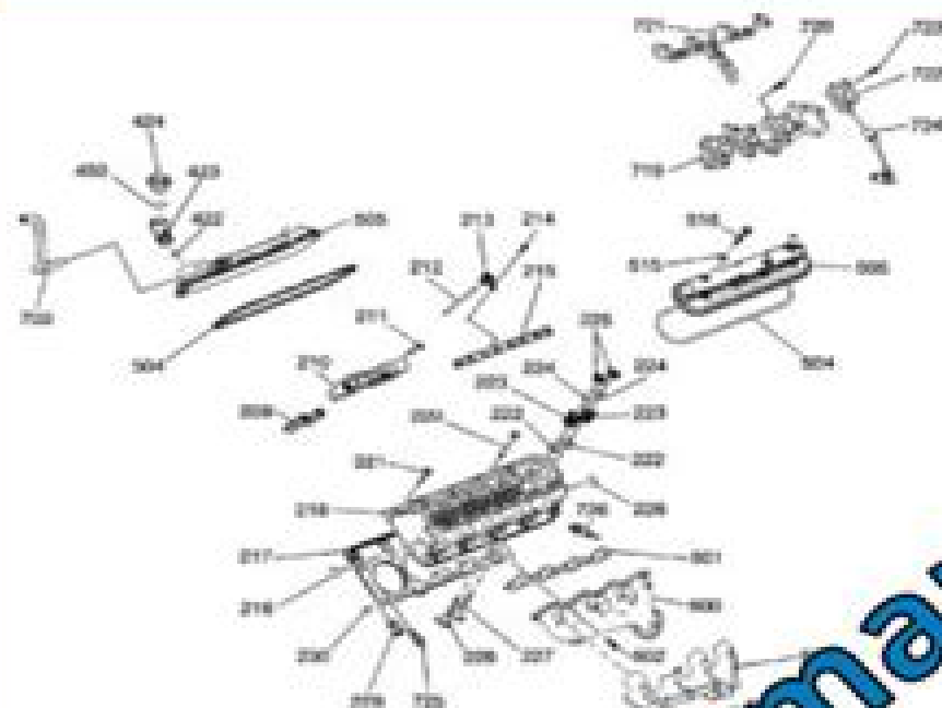
Fig. 12: Cylinder Head/Upper Engine Components Courtesy of GENERAL MOTORS CORP.
